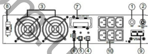
LP Smart-UPS-3000 PRO RM
